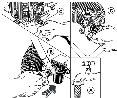
Raccordement hydraulique.
