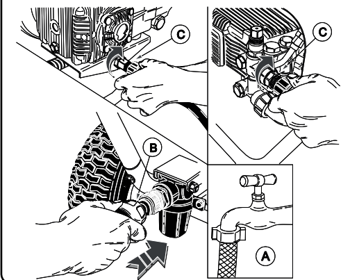
Water circuit connection.
