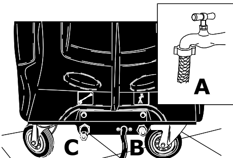
Raccordement hydraulique.
