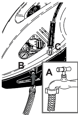
Raccordement hydraulique
